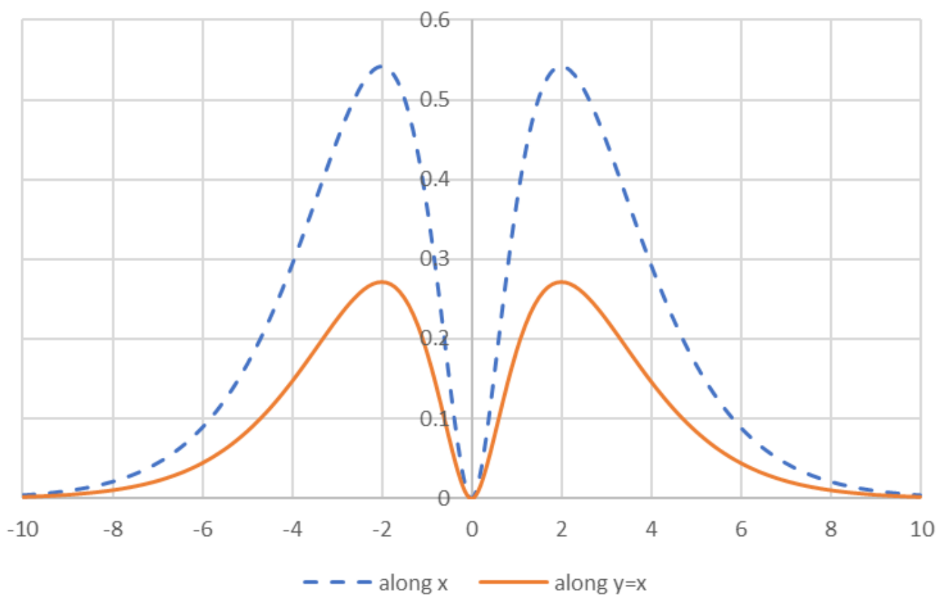
2p_x density
