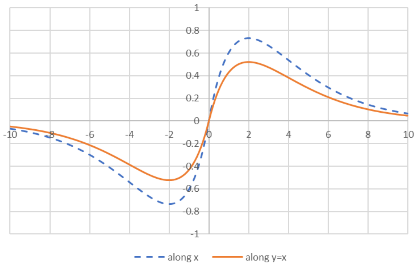
2p_x wave function
